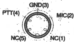
FRONT PANEL VIEW
